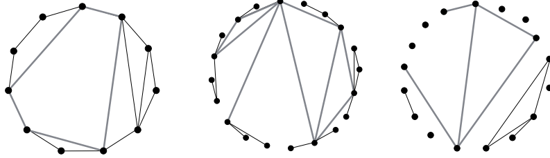
Figure 2: Left: a dissection consisting of a root face (in gray) with an arbitrary dissection glued at each non-root edge. Center: the root of the connected graph belongs to three blocks (in gray); to any other vertex of these blocks there are two connected graphs attached, possibly reduced to a single vertex. Right: between every two consecutive vertices of the root component (in gray) there is an arbitrary graph, possibly empty. In all three cases the root is the vertex on top.
