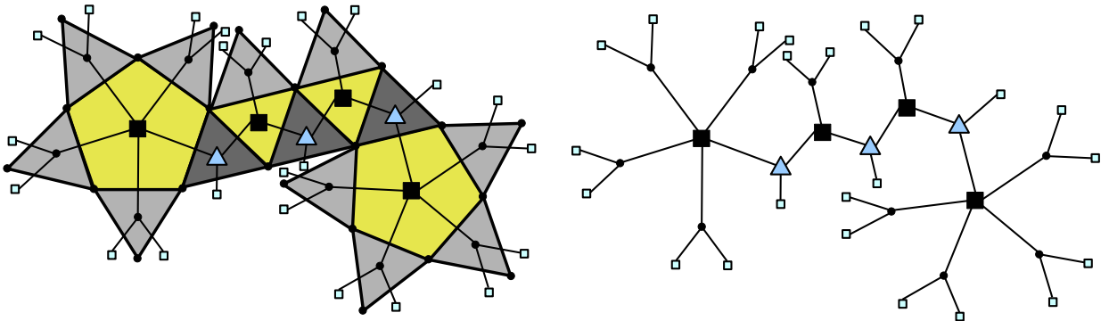
Figure 2: One element of the family and the associated tree. Danglings correspond to vertices of type \square
