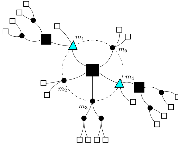
Figure 5: An example, with the geometric circle and the geometric sons
