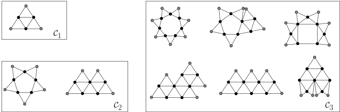
Figure 1: The classes \mathcal{C}_1, \mathcal{C}_2 , and \mathcal{C}_3 .
