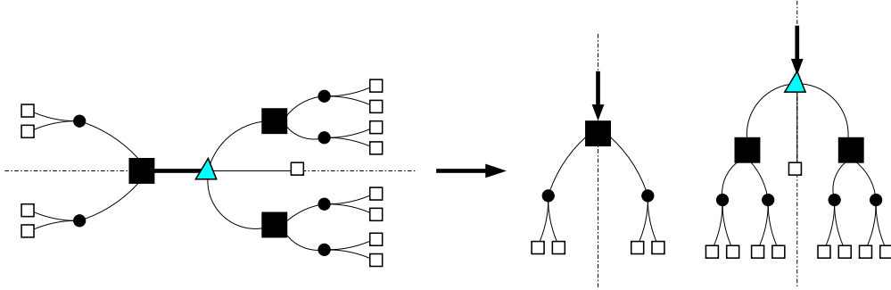
Figure 4: A tree rooted at an edge, and the decomposition into mobiles.
