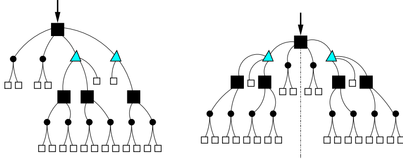
Figure 3: A \blacksquare -mobile and a symmetric \blacksquare -mobile.
